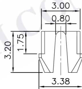
DETAIL X
